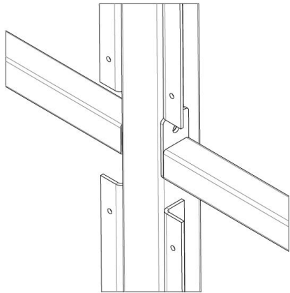
5mm CLAMP PLATE w/ FOURTRESS M8X50mm SECURITY SCREW
