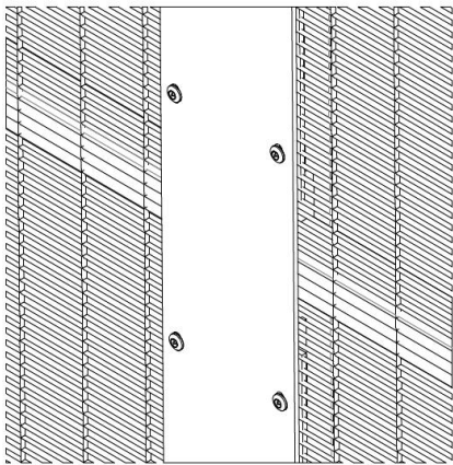
5mm CLAMP PLATE w/ FOURTRESS M8X50mm SECURITY SCREW
