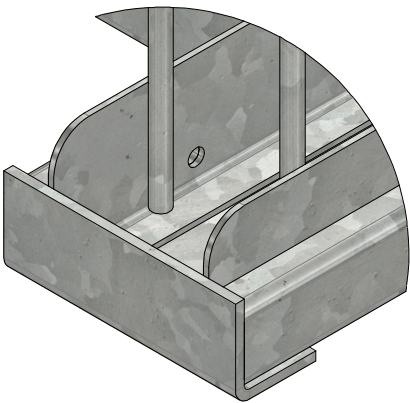
IMPROVED END PLATE Y ( 1:3 )
