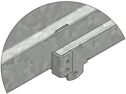
IMPROVED END PLATE Y ( 1:3 )
